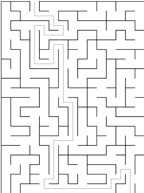
Maze 67
