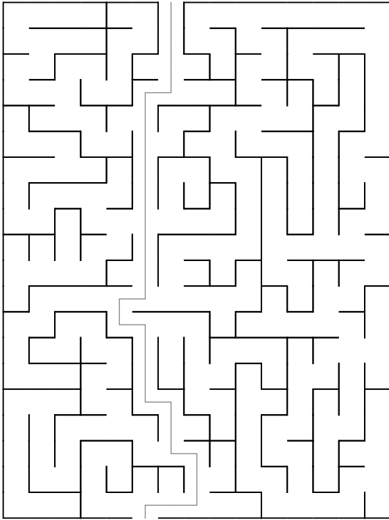
Maze 73
