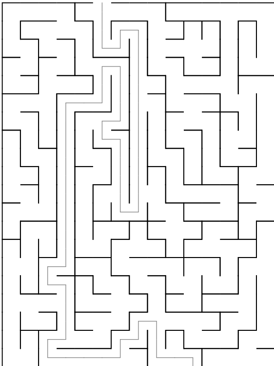
Maze 31
