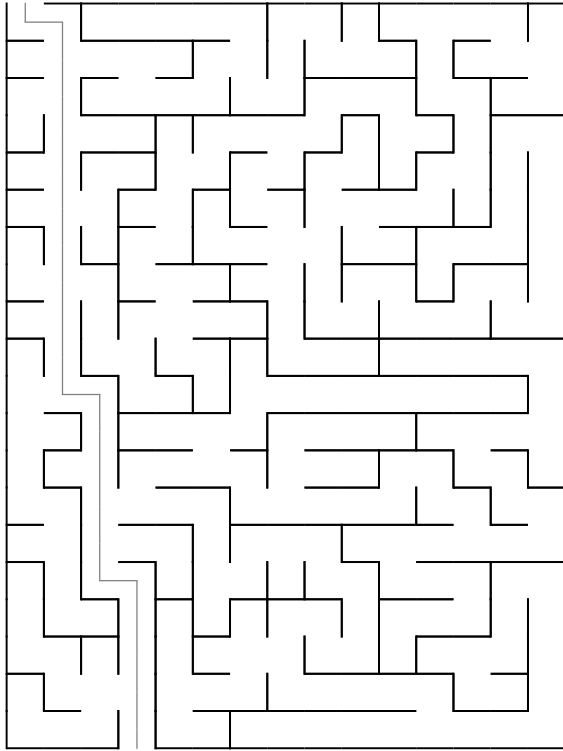
Maze 33
