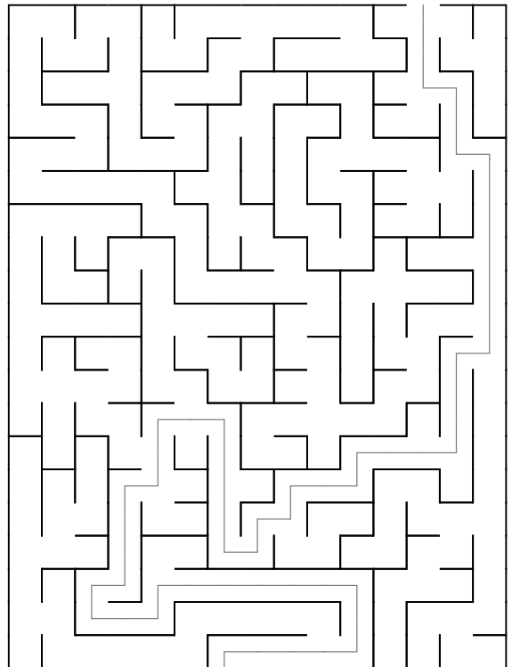
Maze 44
