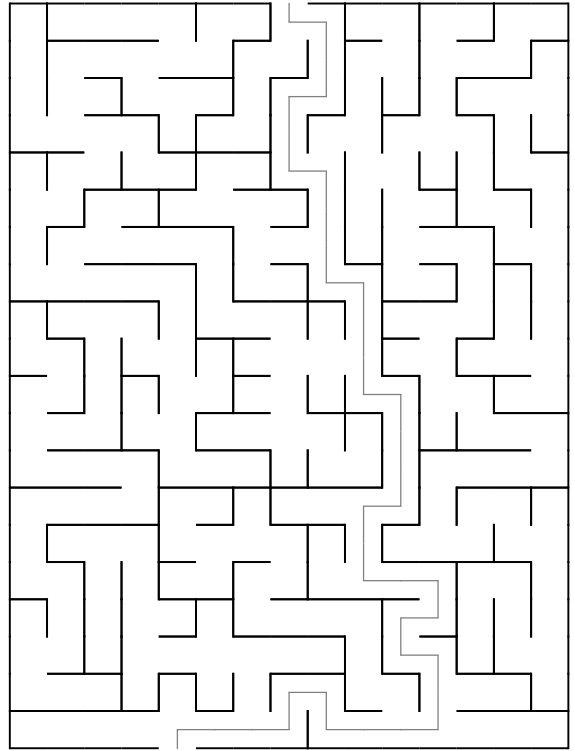
Maze 34
