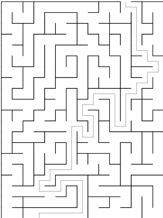
Maze 83
