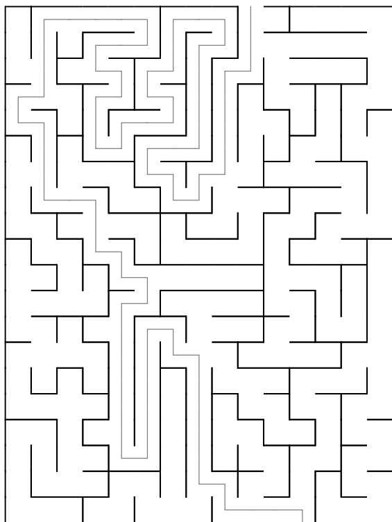
Maze 61
