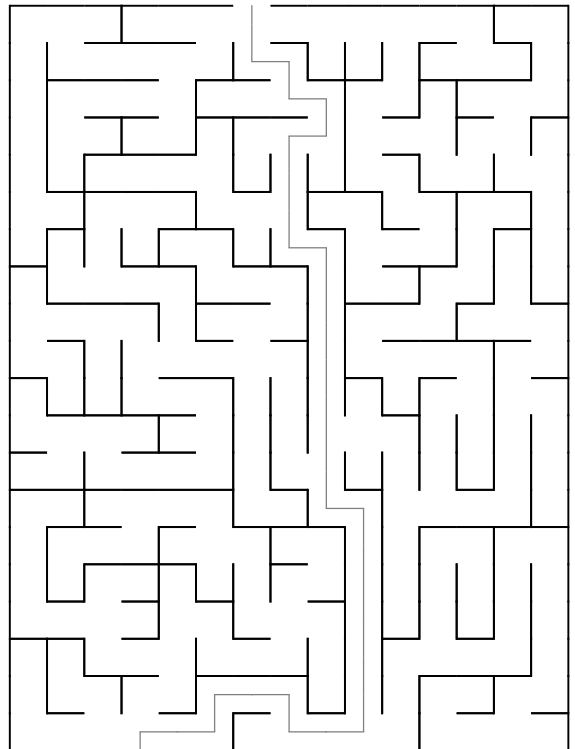
Maze 16
