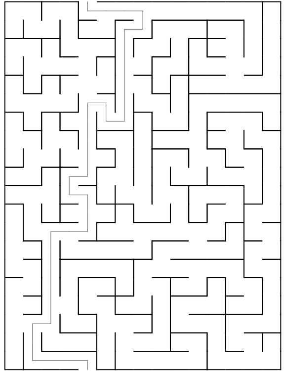
Maze 94
