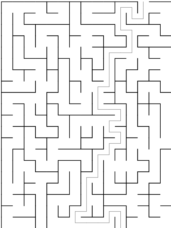
Maze 51
