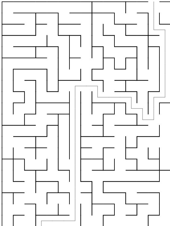
Maze 35
