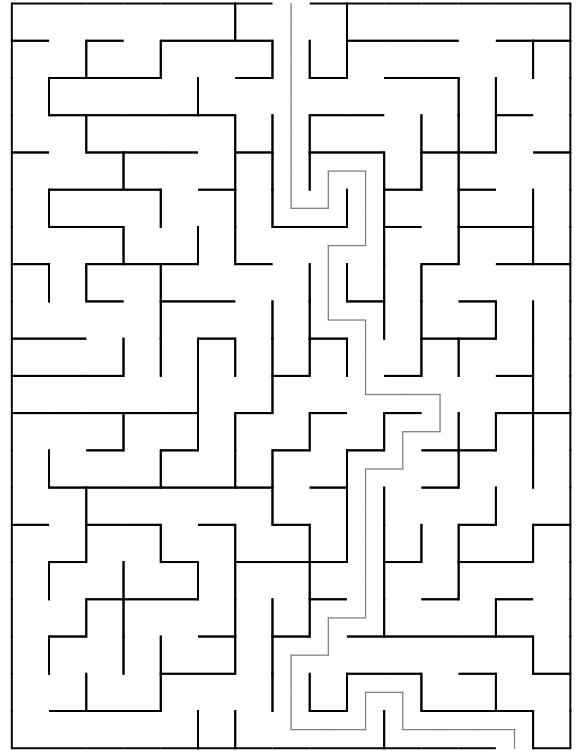
Maze 74
