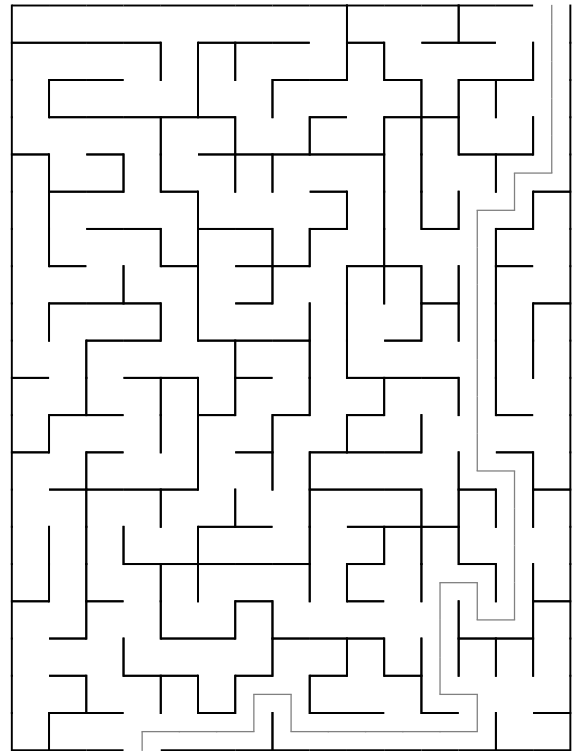
Maze 10
