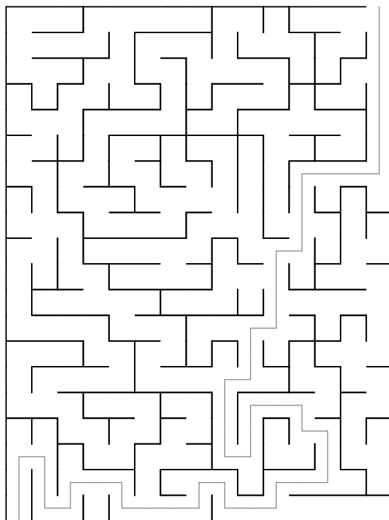
Maze 80
