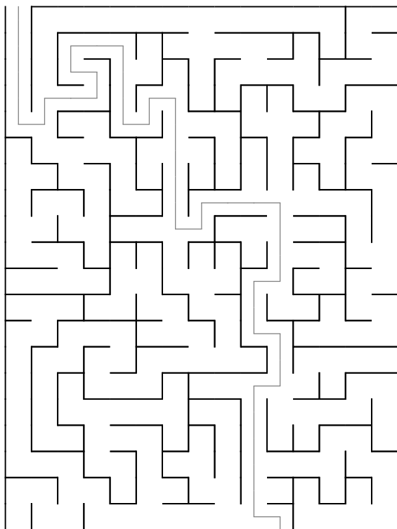
Maze 57
