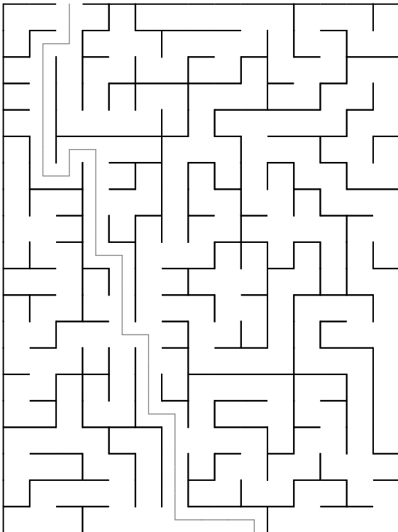
Maze 3
