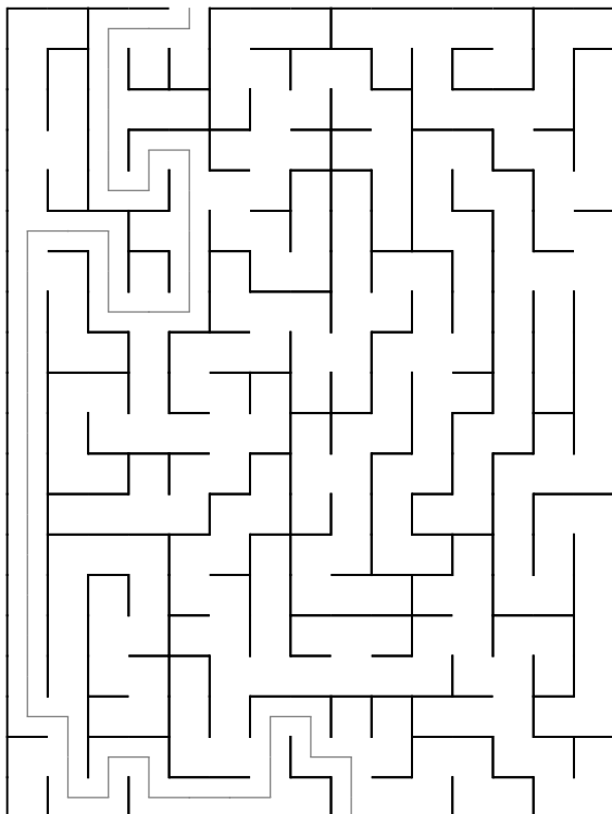
Maze 11
