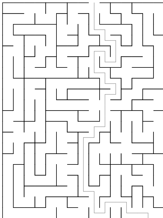
Maze 78
