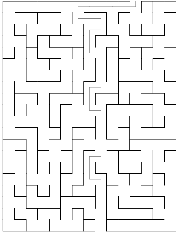
Maze 46
