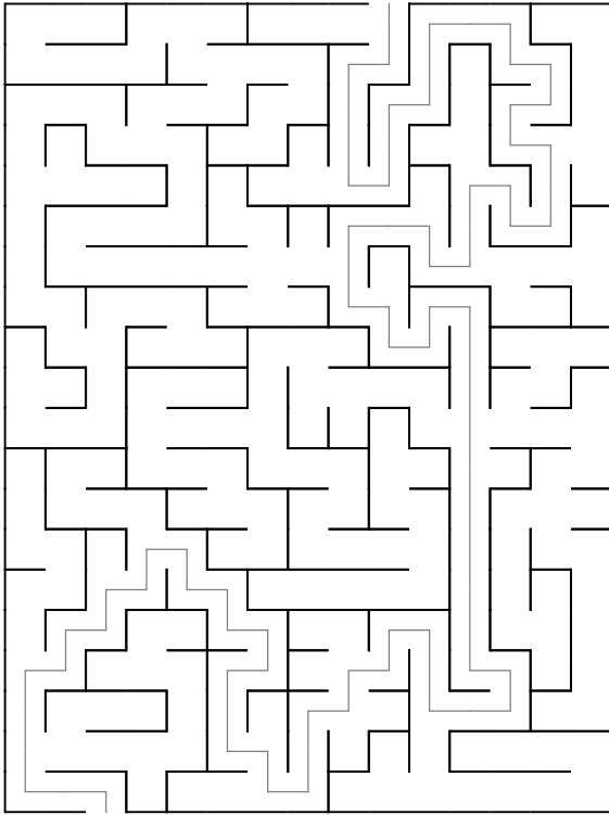
Maze 21
