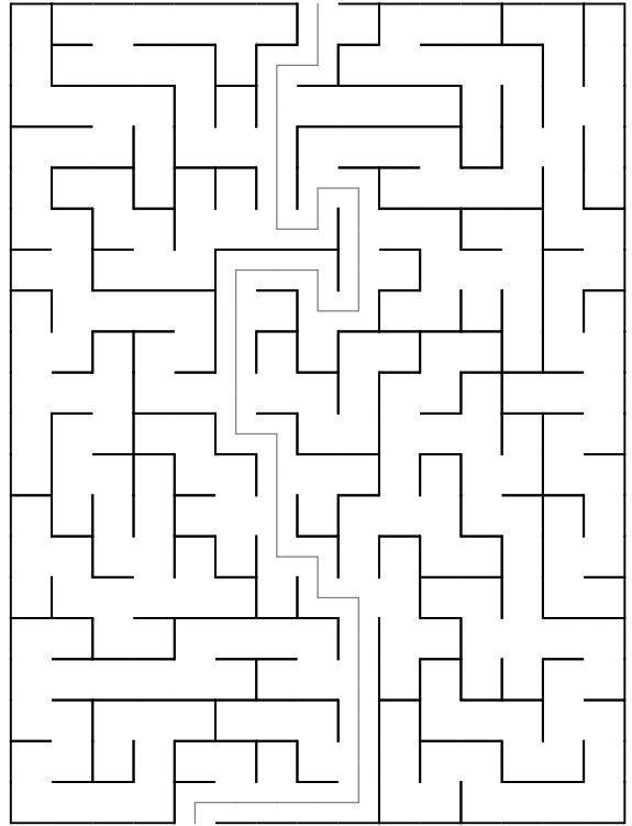
Maze 14
