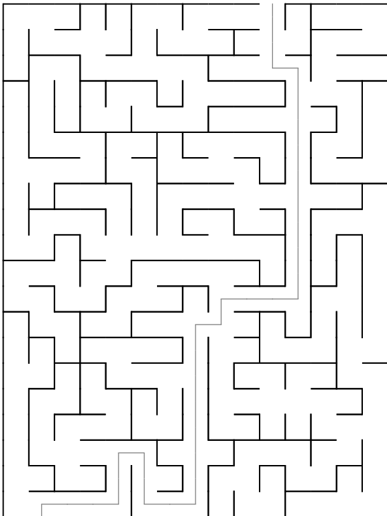
Maze 7
