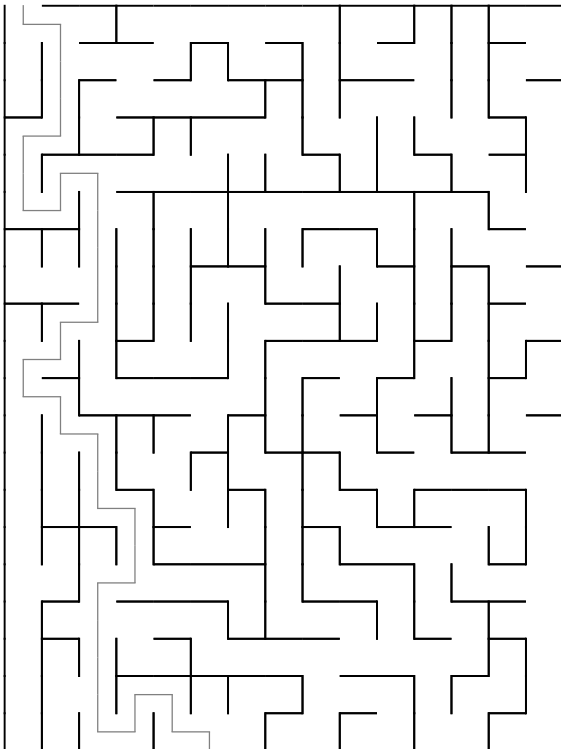
Maze 55
