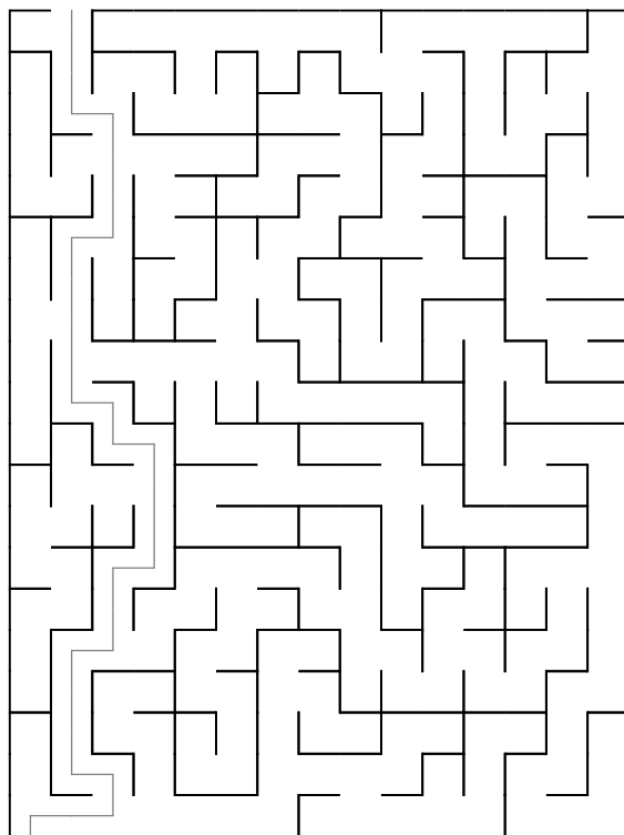
Maze 58
