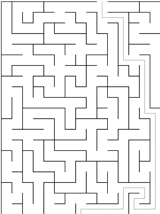
Maze 75
