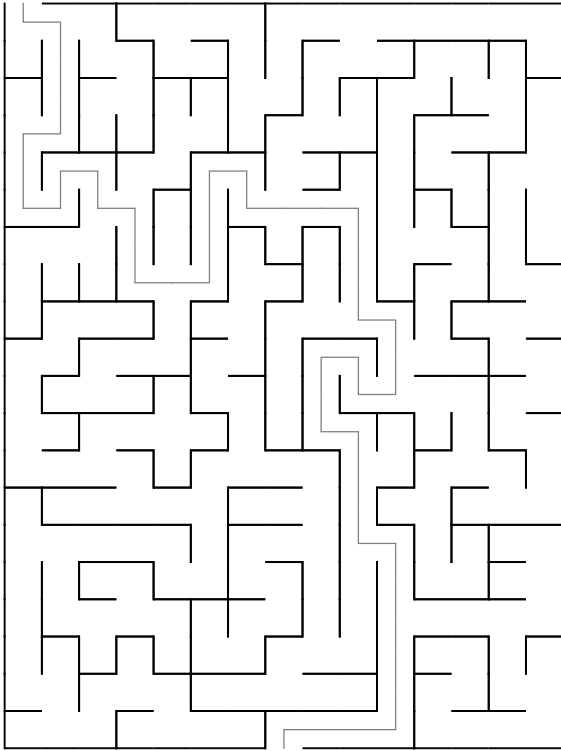
Maze 81
