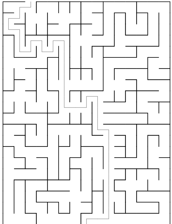
Maze 36
