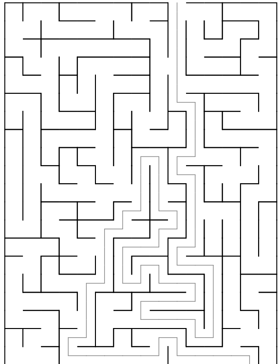
Maze 96
