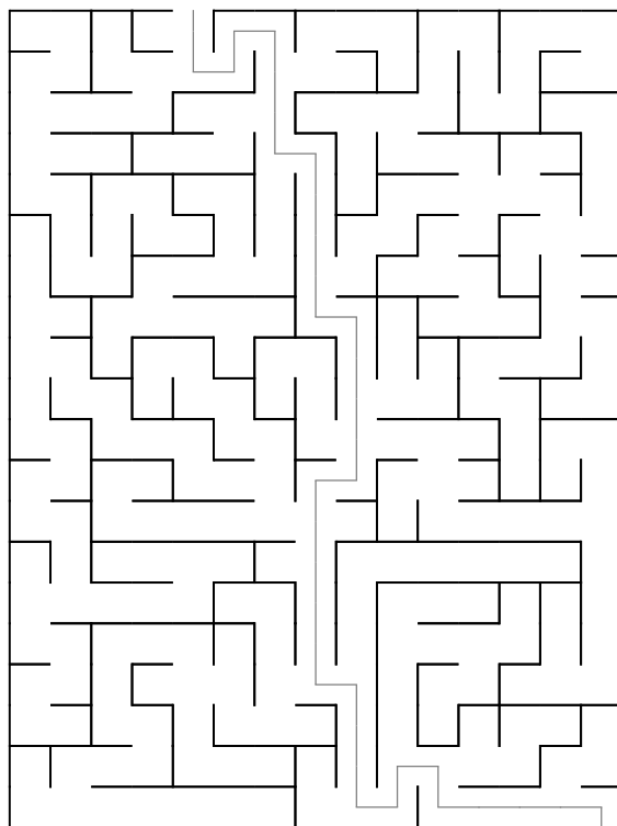
Maze 60
