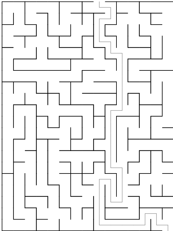
Maze 9
