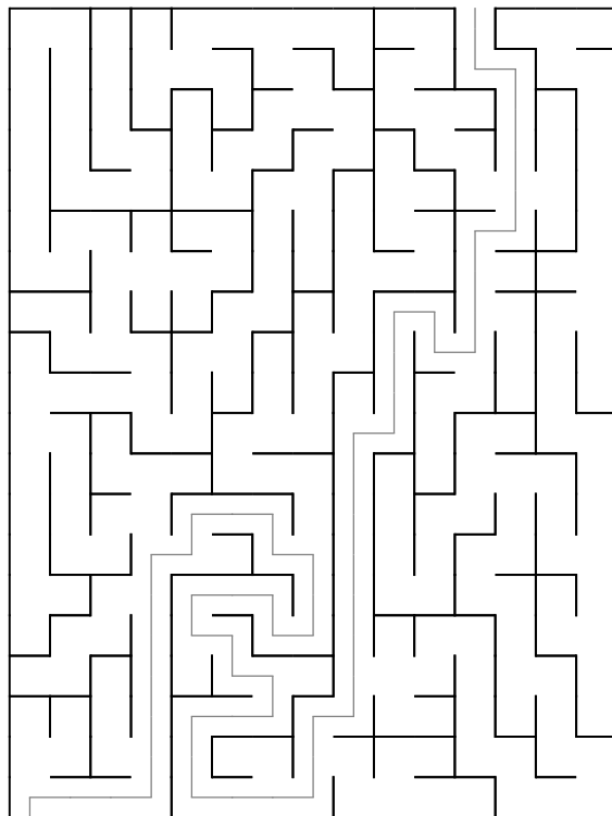
Maze 100
