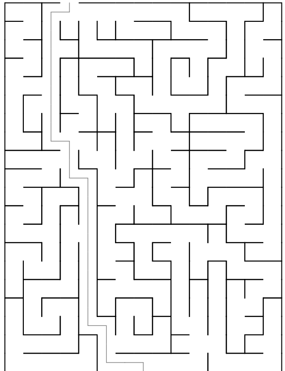
Maze 72
