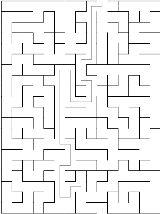
Maze 65
