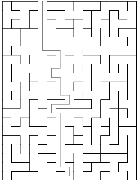
Maze 8
