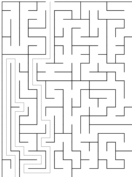
Maze 98
