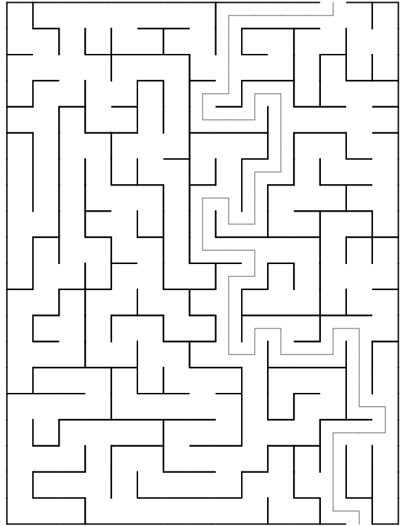
Maze 86
