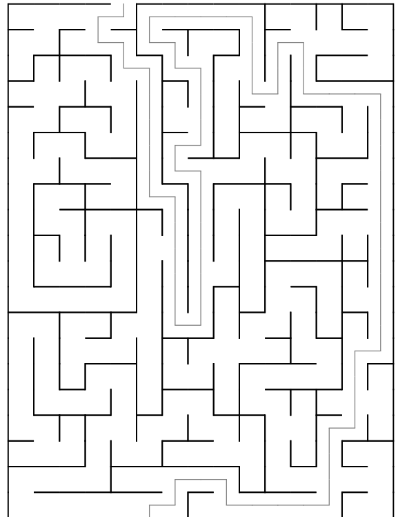
Maze 56
