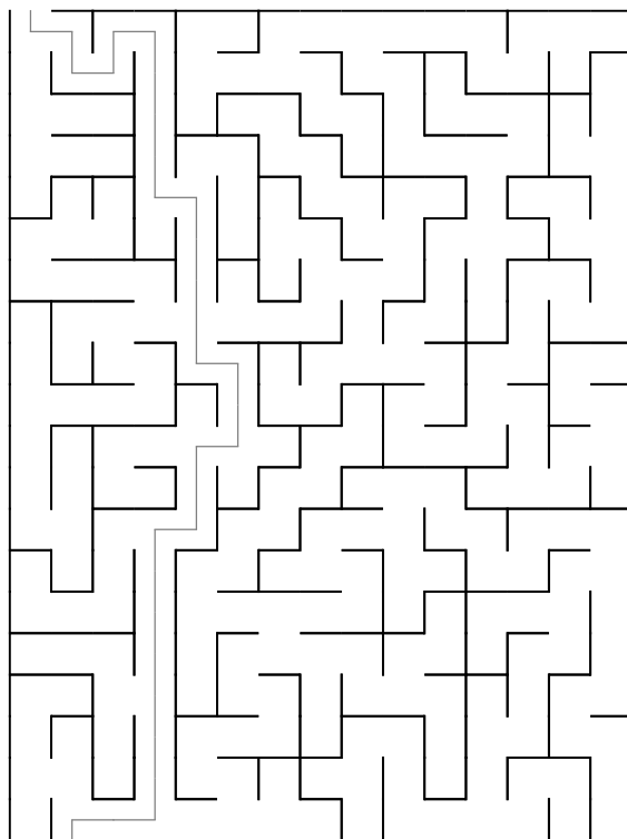
Maze 92
