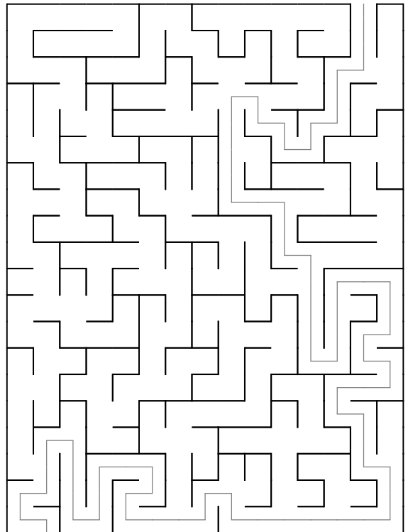
Maze 24
