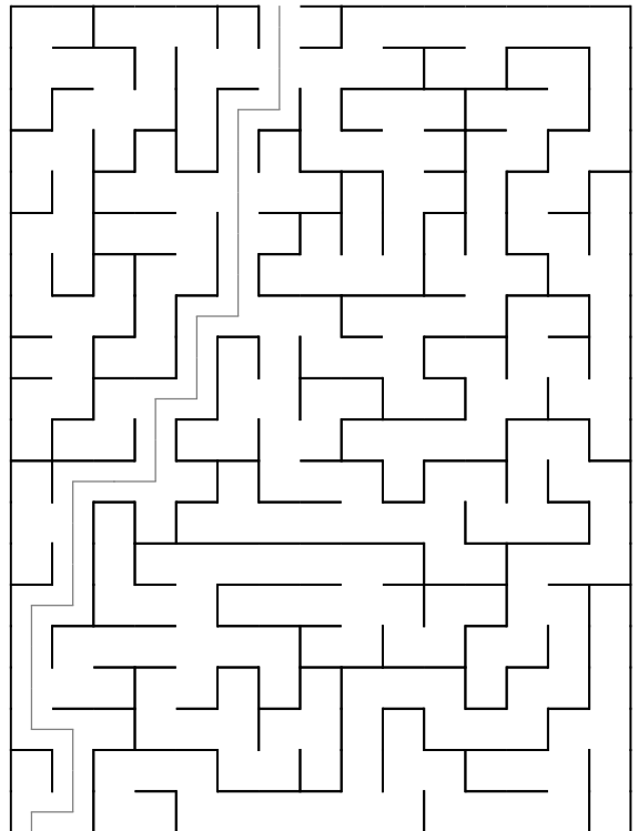
Maze 4
