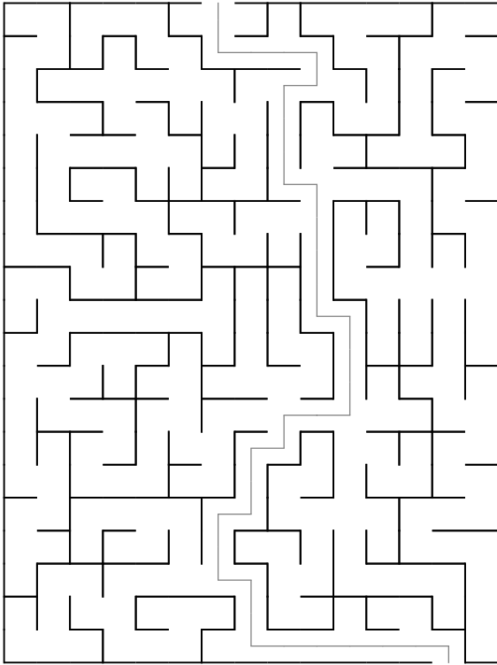
Maze 29
