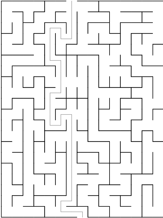
Maze 53
