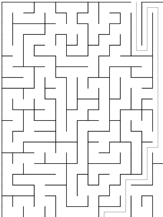
Maze 97
