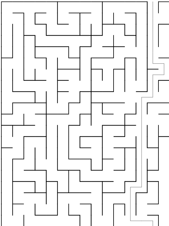
Maze 27
