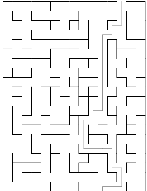
Maze 76
