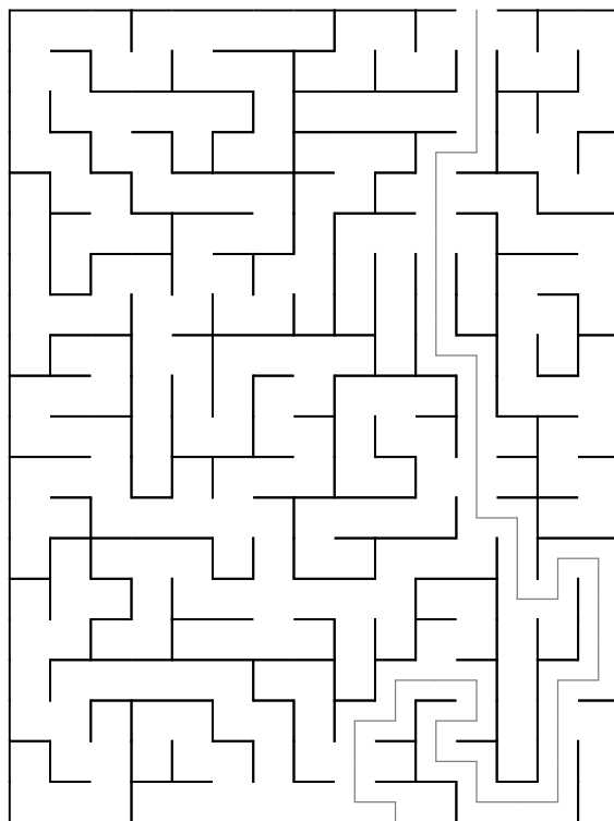
Maze 62
