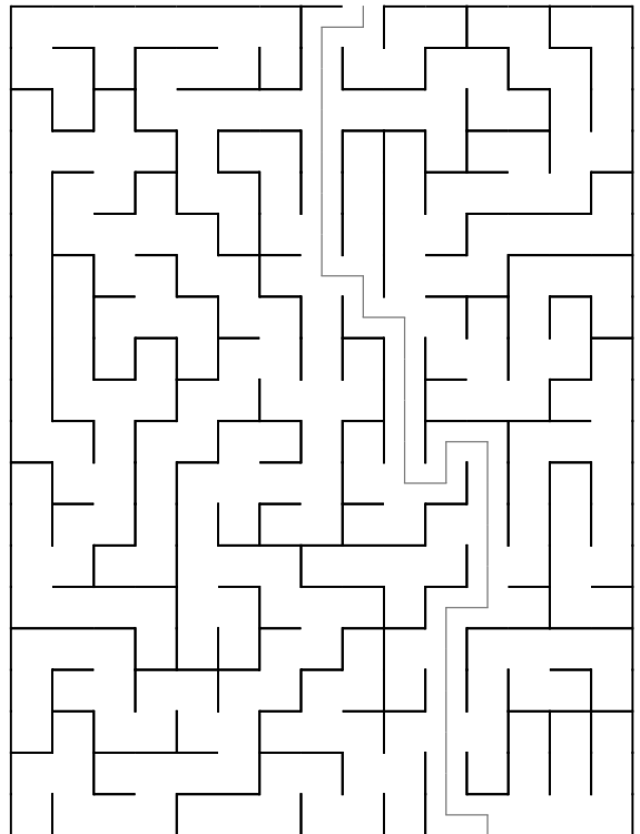
Maze 32
