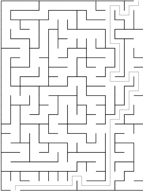
Maze 45
