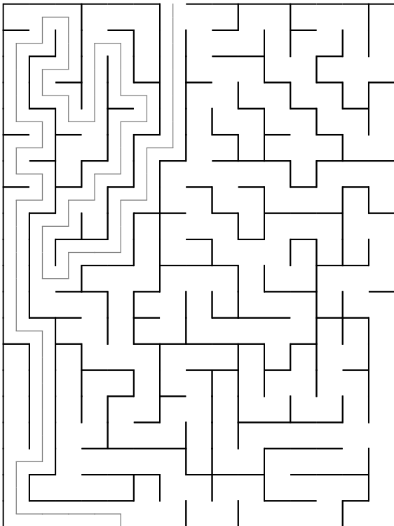
Maze 43
