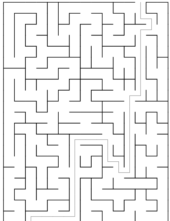
Maze 12
