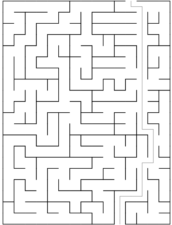
Maze 50
