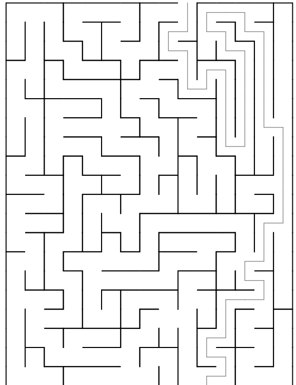
Maze 68
