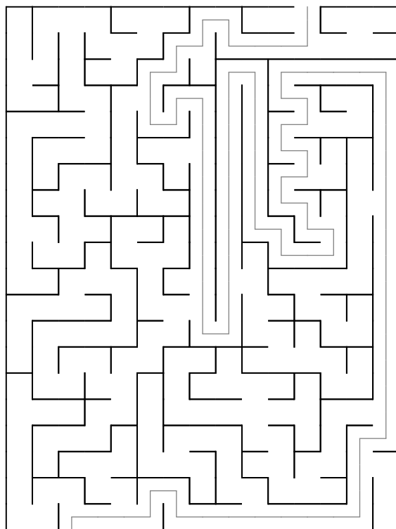
Maze 64
