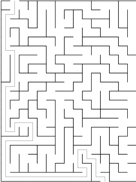
Maze 13
