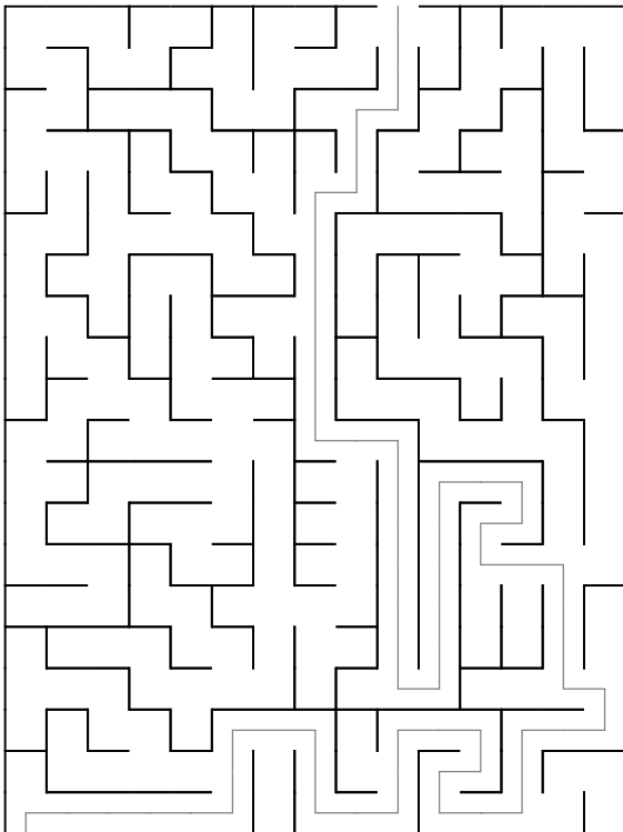
Maze 95
