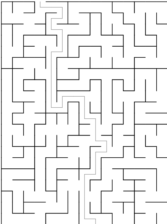
Maze 15
