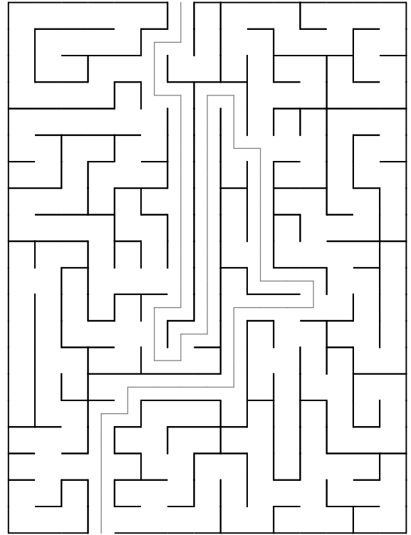
Maze 26
