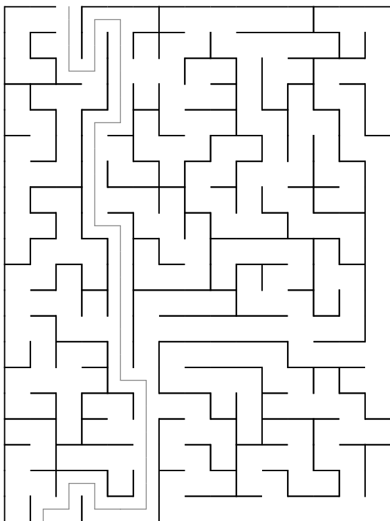
Maze 79
