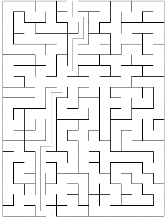
Maze 2
