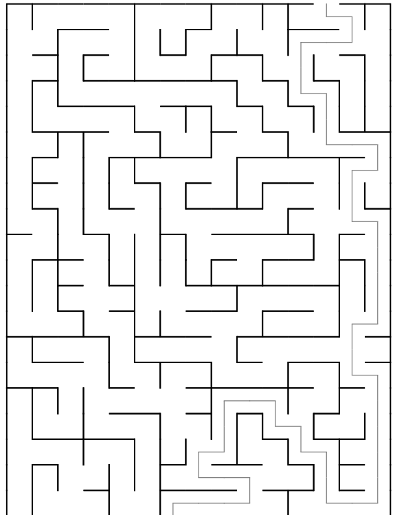
Maze 52
