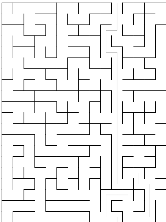
Maze 91
