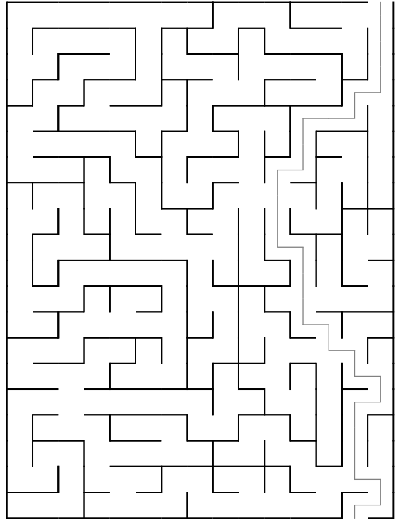
Maze 38
