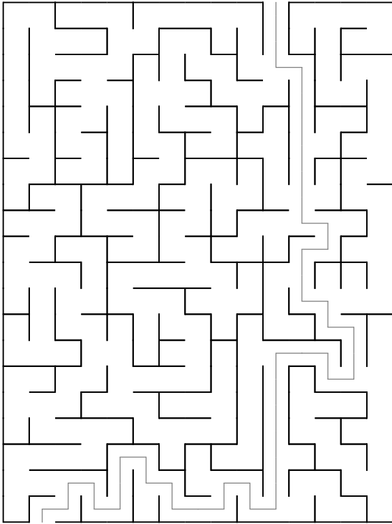
Maze 41
