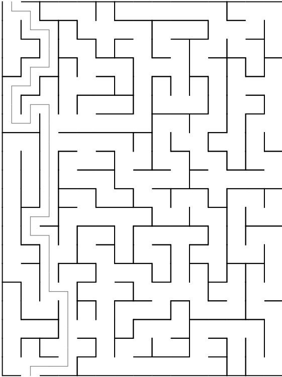
Maze 69
