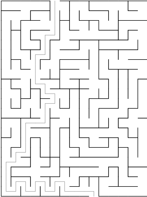
Maze 1
