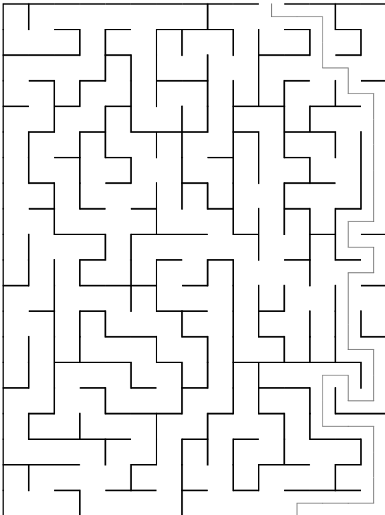
Maze 23
