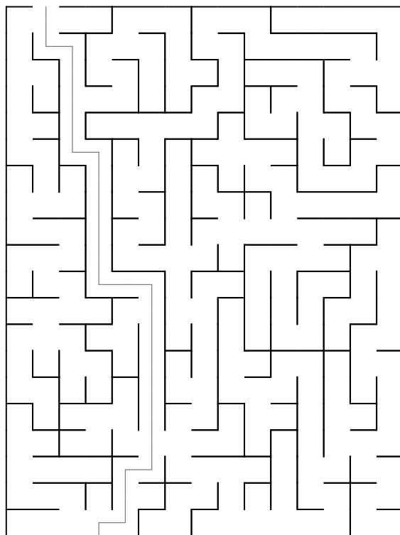
Maze 90
