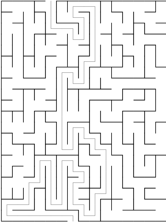
Maze 25
