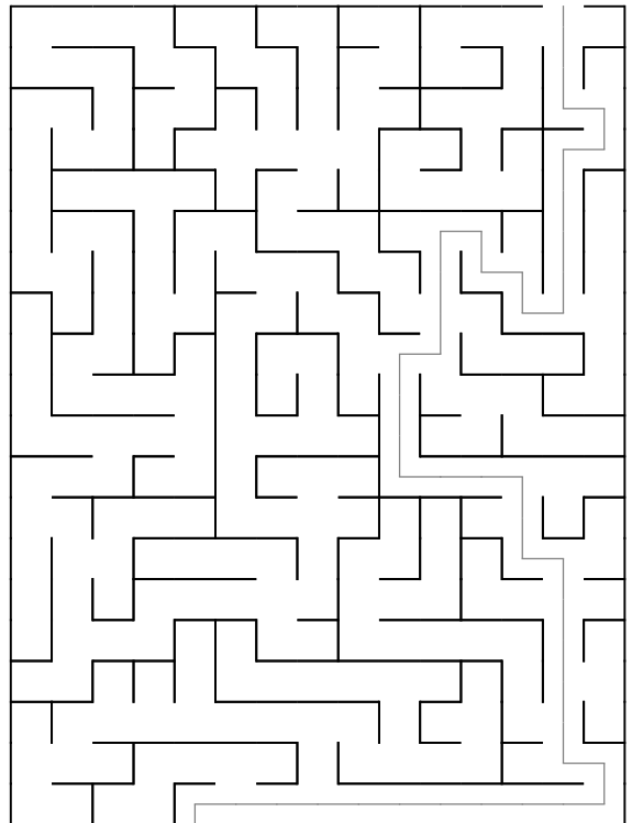
Maze 84
