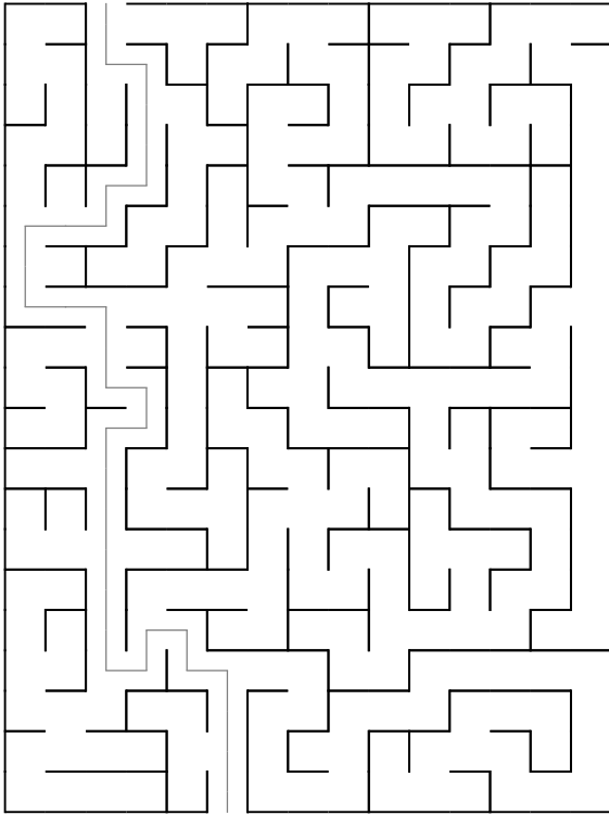
Maze 85
