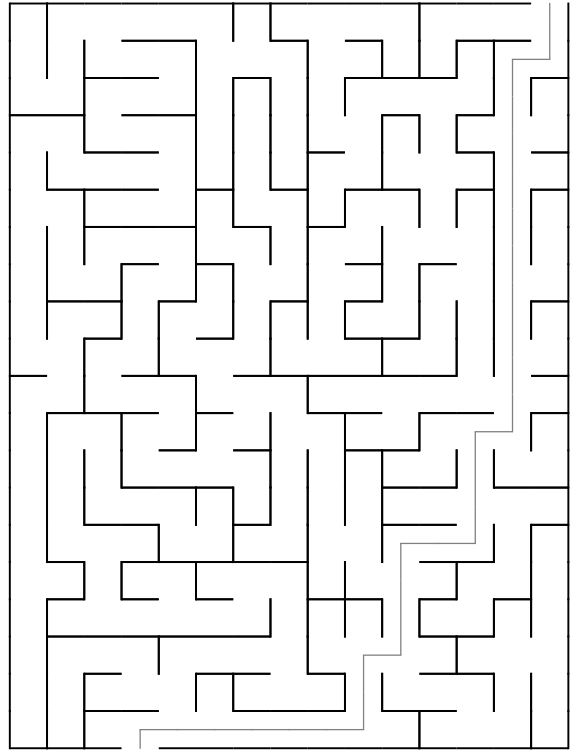
Maze 22
