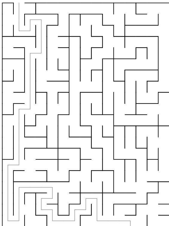
Maze 63
