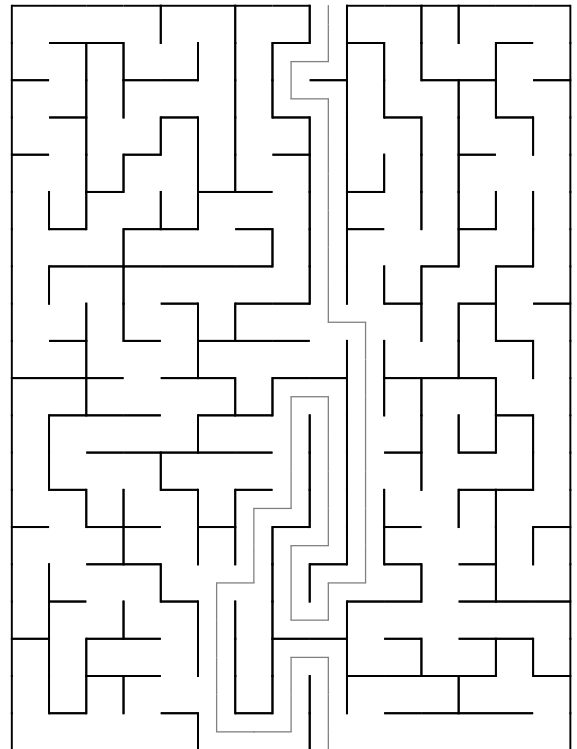
Maze 28
