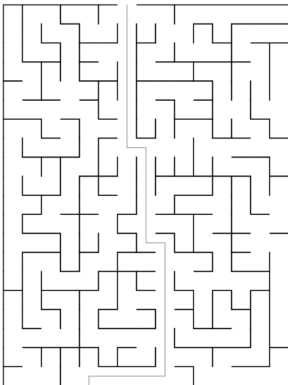
Maze 77
