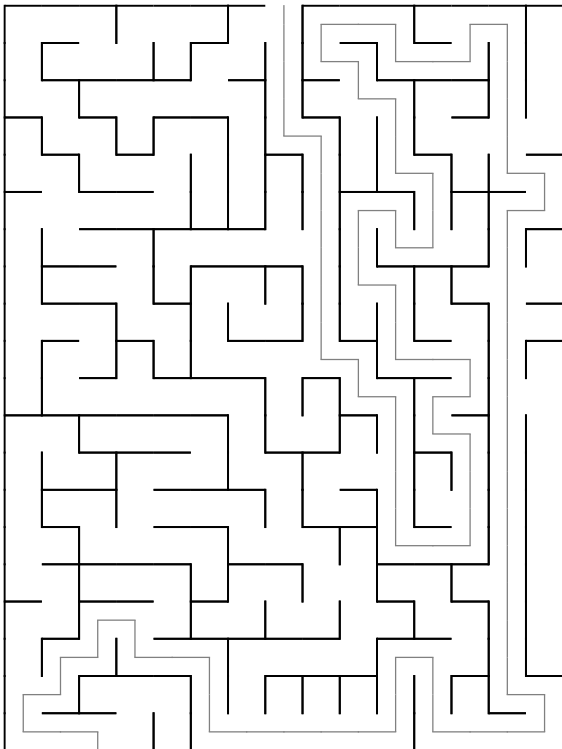
Maze 39
