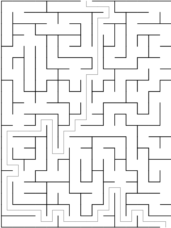
Maze 5
