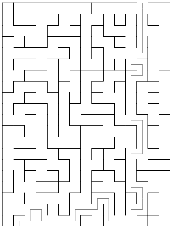
Maze 59
