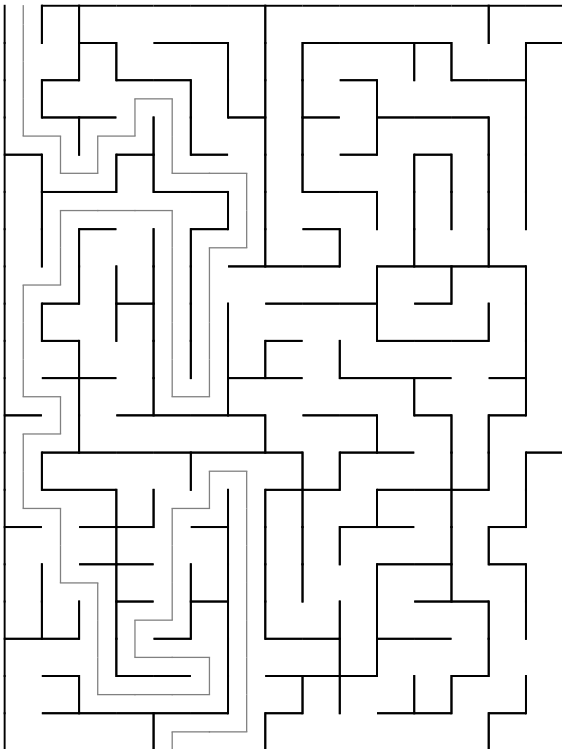
Maze 47
