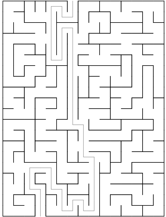
Maze 42
