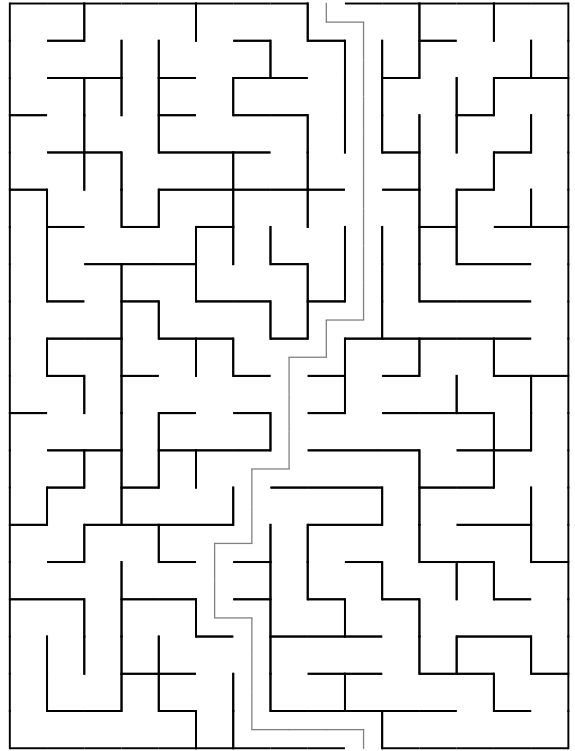
Maze 30
