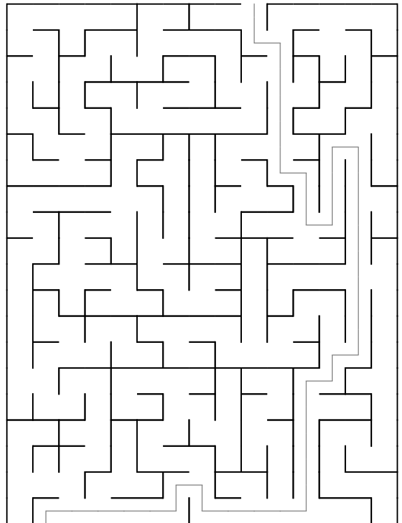
Maze 48
