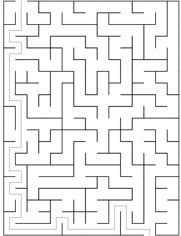
Maze 54
